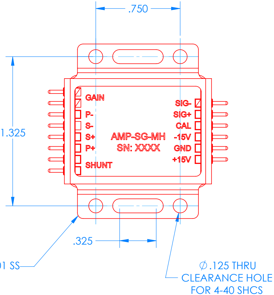
BOLT PATTERN FOR FLAT SURFACE MOUNTING
